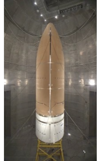
Ariane 5 fairing separation test
